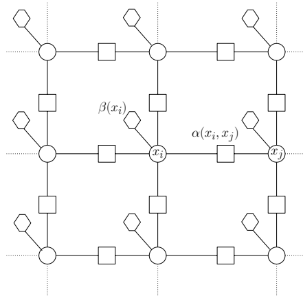
Figure 2. Illustration of our graphical model. The circles represent pixels while squares and hexagons denote the factors capturing the pair-wise interaction and unary potentials, respectively
