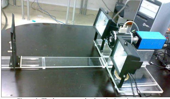
Figure 1. The hyperspectral palmprint imaging system.
